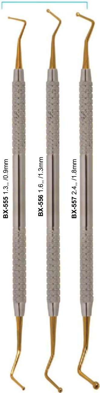
FILLING INSTRUMENTS ball 6mm length 170mm
